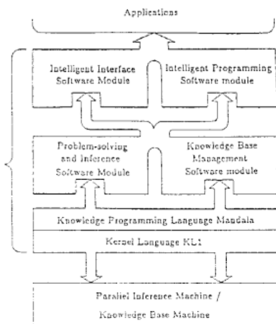
Fig. 2 The basic software system
