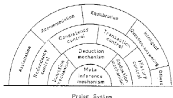
Fig. 4 The knowledge acquisition module
