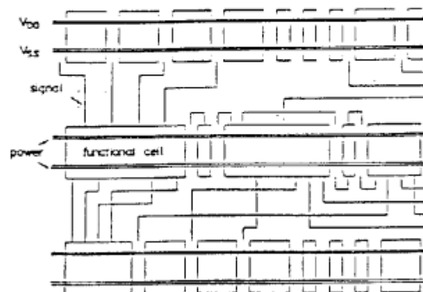
Figure 16. Example of a row-based layout scheme.
