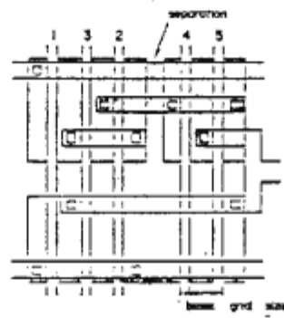
Figure 11. Optimization of layout.
