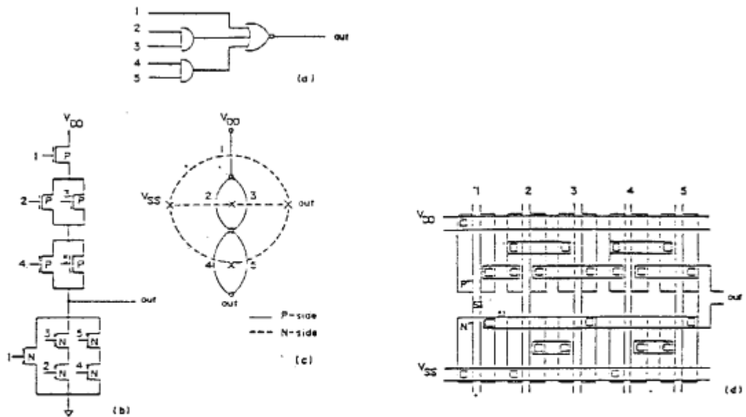
Figure 10. Basic layout of the functional cell. (a) Logic diagram (b) Circuit (c) Graph model (d) Layout
