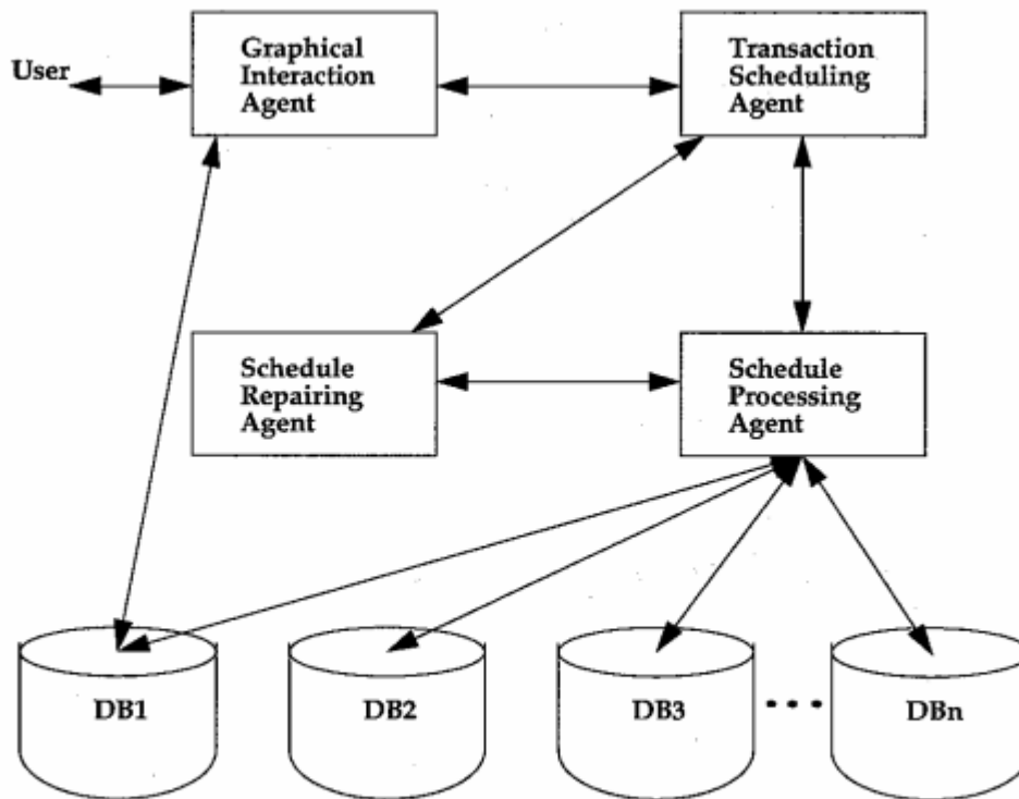
Figure 3: Agents used for relaxed transaction processing
