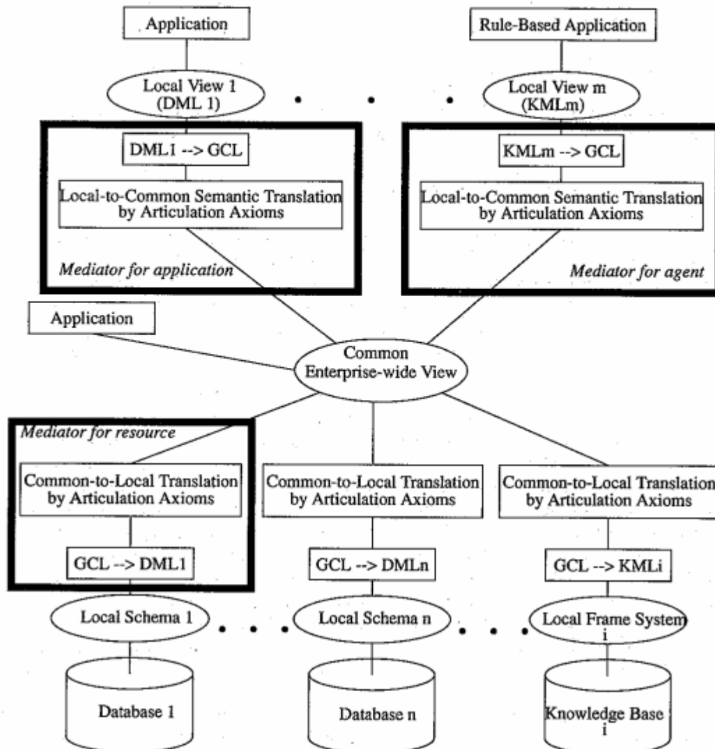
Figure 2: Logical view of the execution environment, showing how mediating agents apply articulation axioms to achieve semantic interoperability
