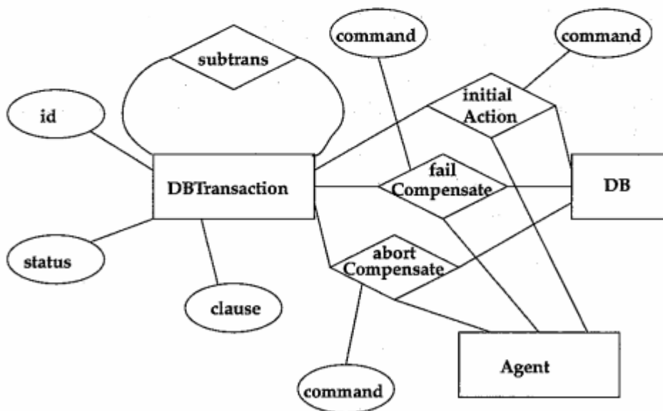
Figure 9: Semantic model for the schedule-repairing agent
