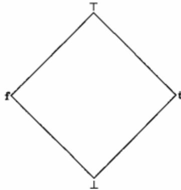
Figure 1. Four-valued logic
