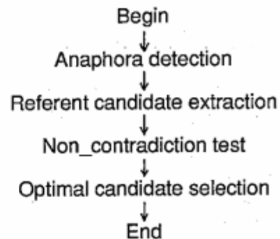
Figure 4 Interpreting input message process flow.
