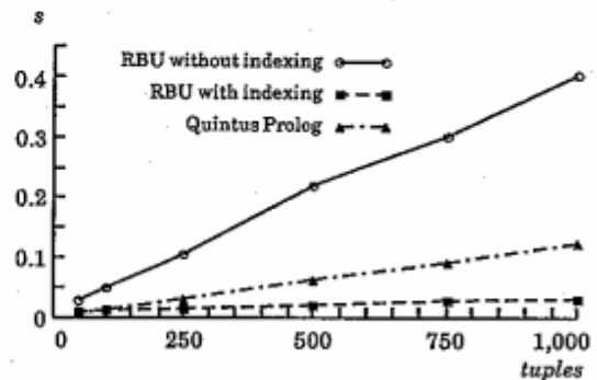
Figure 19. Comparison of search speeds
