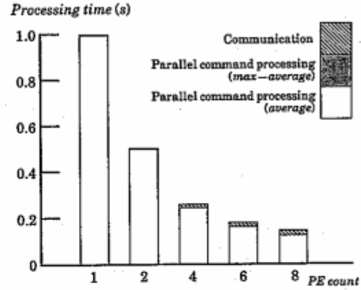
Figure 13. Performance of the selection operation
