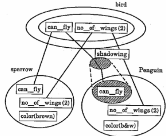
Figure 4. Inheritance in knowledge bases
