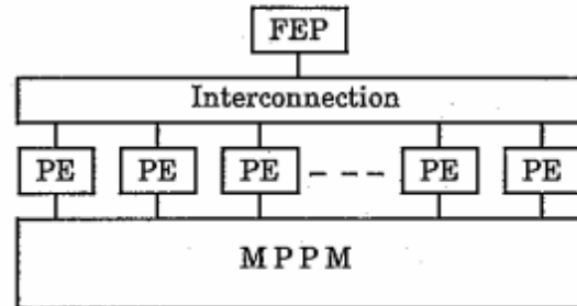
Figure 10. Hardware configuration of the parallel knowledge base system
