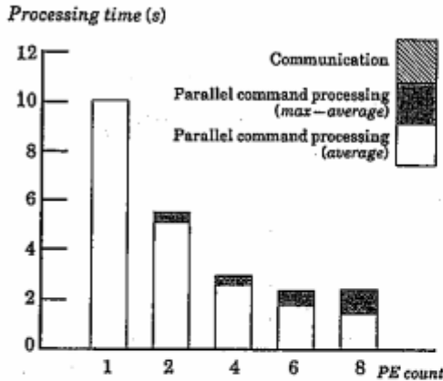
Figure 14. Performance of the join operation
